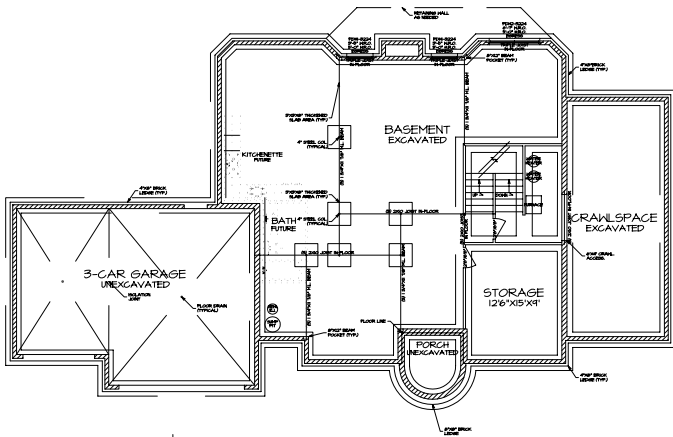
FOUNDATION PLAN A-4 SCALE: 1/4"=1'-0"
