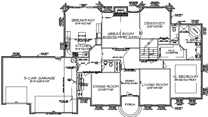
FIRST FLOOR PLAN A-3 SCALE: 1/4"=1'-0"
